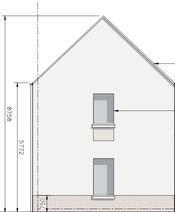
GABLE ELEVATION (Render)
