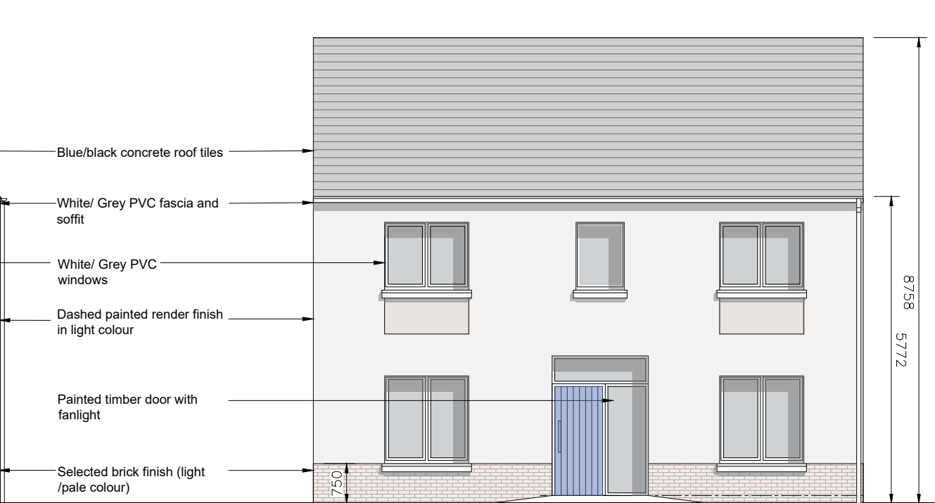
FRONT ELEVATION (Render)
