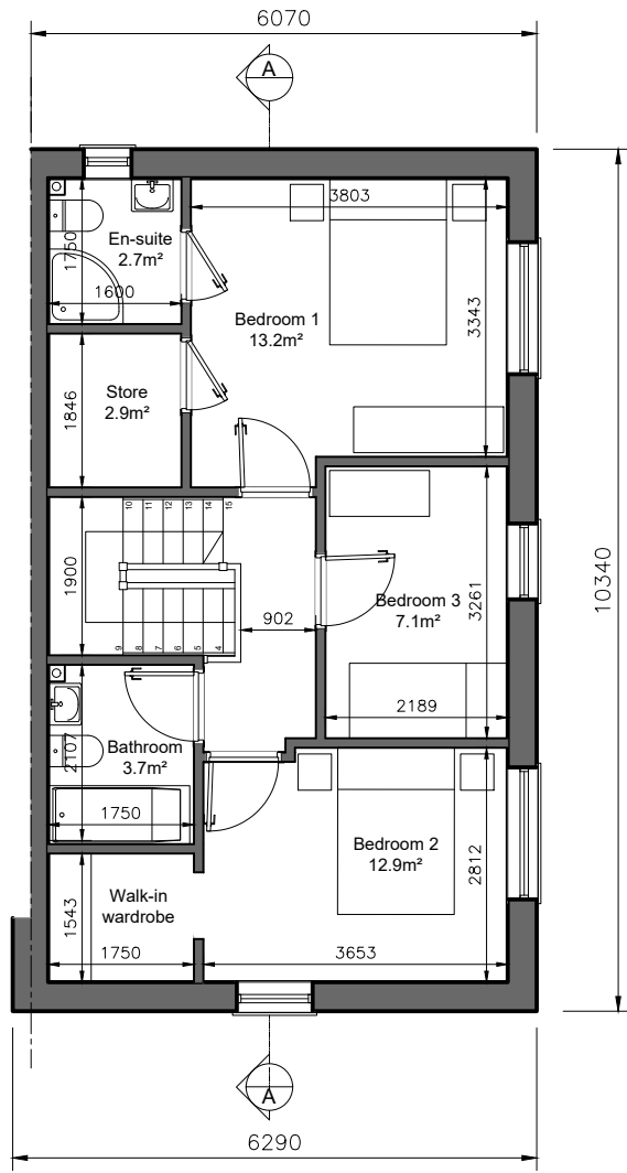
FIRST FLOOR PLAN 53.2m 2
