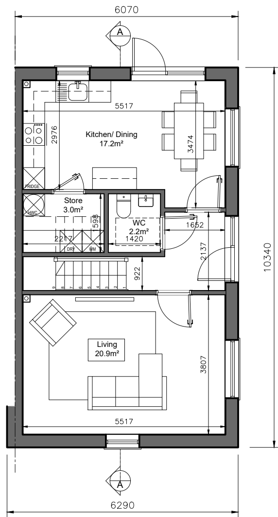
GROUND FLOOR PLAN 53.2m 2 TOTAL FLOOR AREA 106.4m 2
