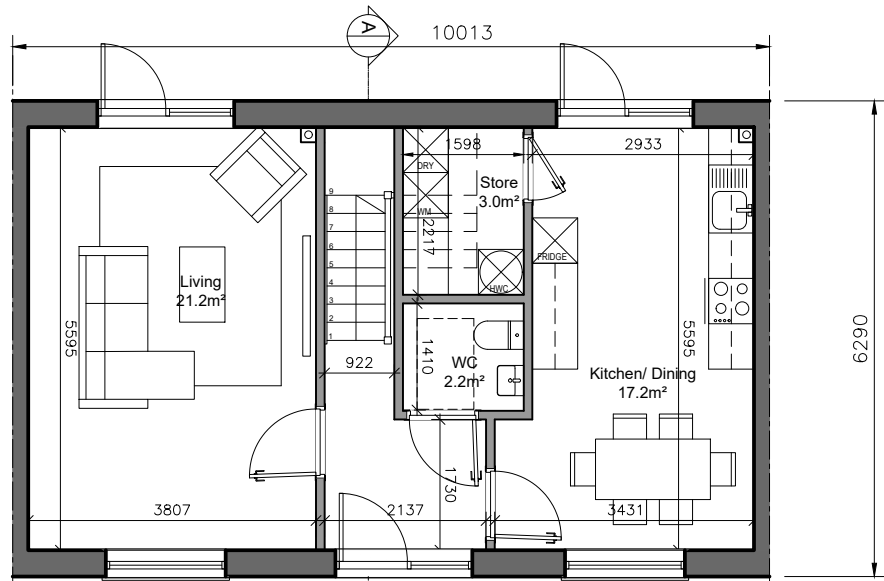
GROUND FLOOR PLAN 53.7m² TOTAL FLOOR AREA 107.4m²
