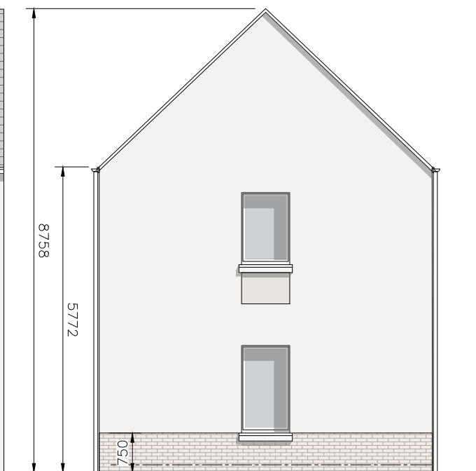
GABLE ELEVATION (Render)
