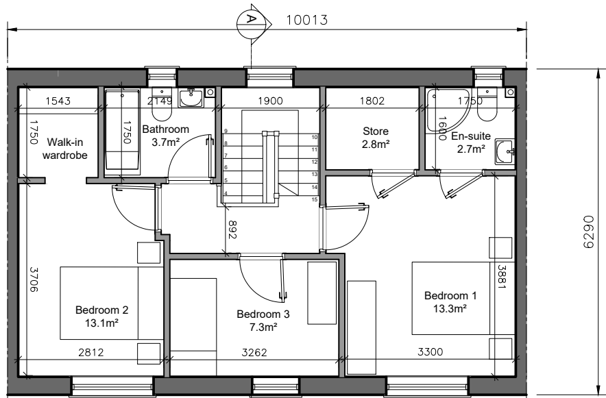
FIRST FLOOR PLAN 53.7m²
