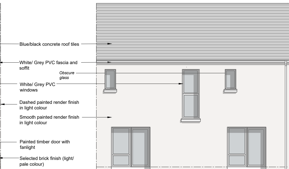
REAR ELEVATION
