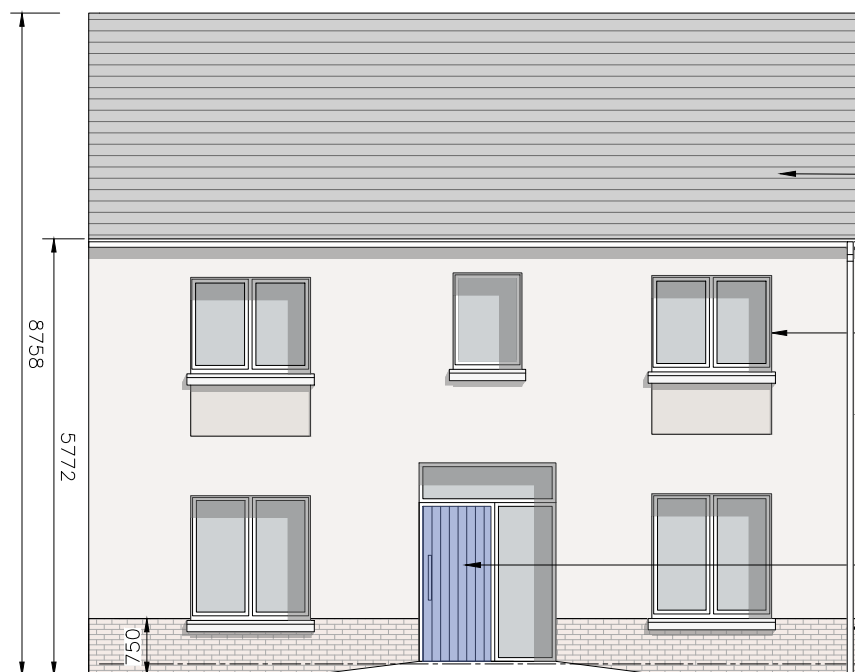
FRONT ELEVATION (Render)
