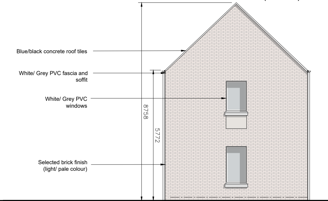
GABLE ELEVATION (Brick)
