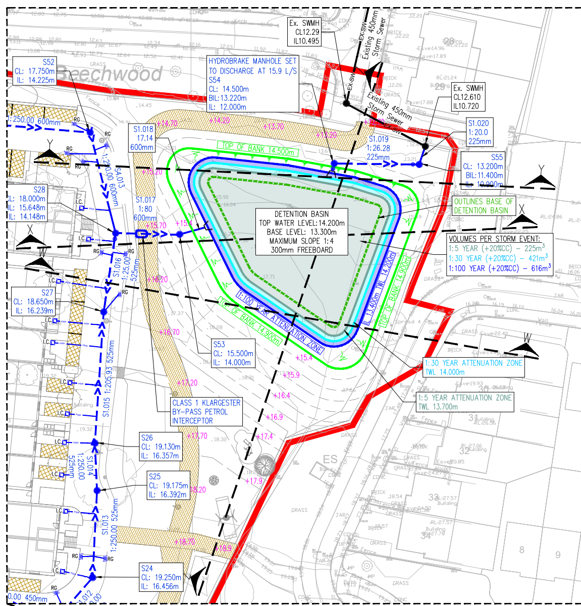
DETENTION BASIN FOCUSED AREA
