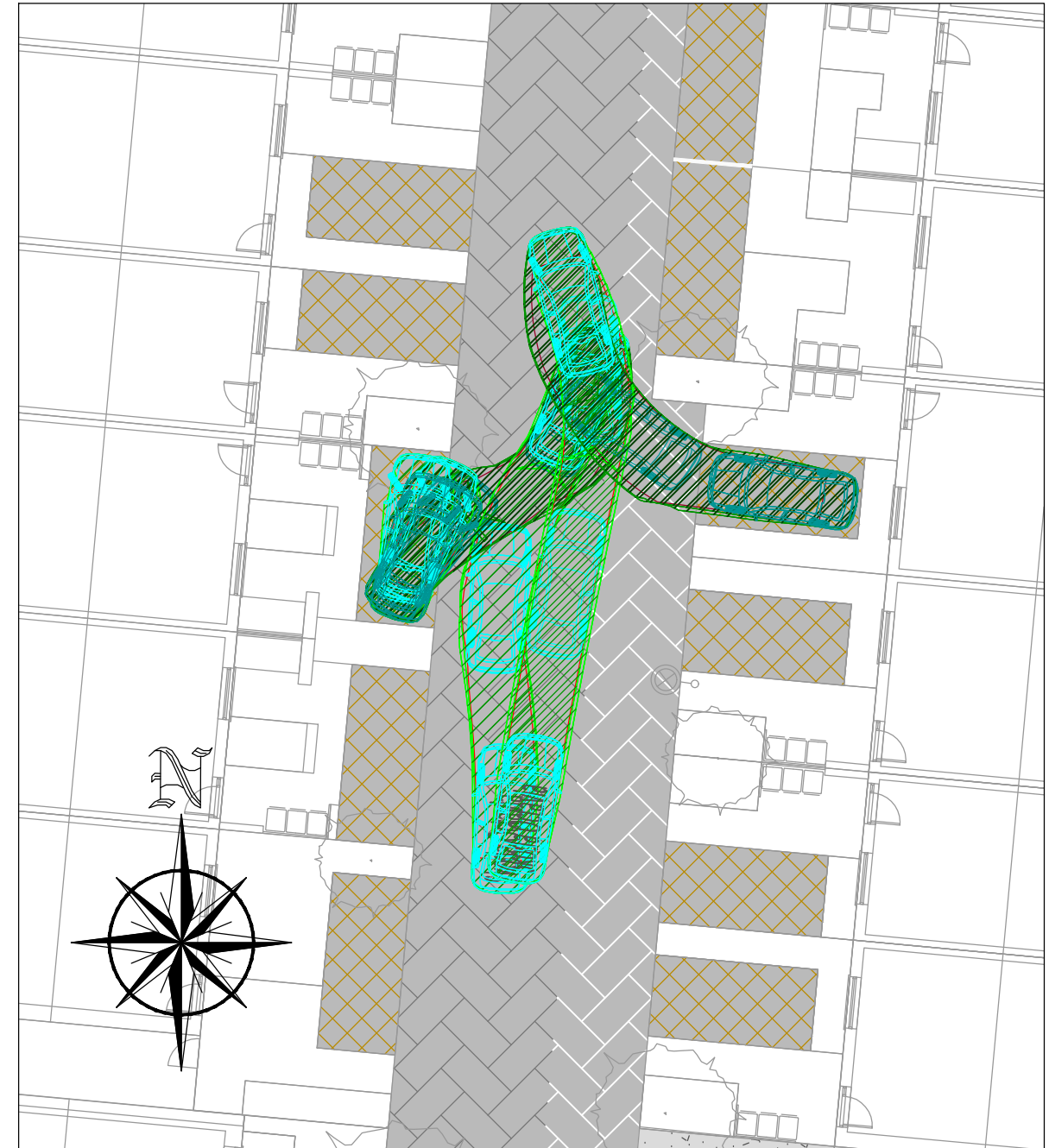
VIEW 11. SCALE 1:200
